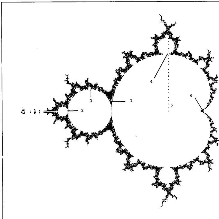
Fig. 7. Display of the Mandelbrot set in the complex plane (Real = -2.0 to 0.5 and Imaginary = -1.25 to 1.25), showing the location of the c values chosen for various iterated maps shown in the corresponding figure numbers. The vertical dotted line is the track of the orbits displayed in Fig. 5.
